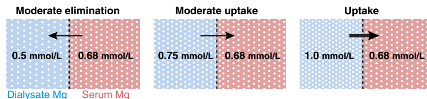
Fig. 4. Dialytic magnesium removal or uptake is dependent on the dialysate-serum magnesium gradient (here based on a total serum magnesium concentration of 1.05 and an ionized (i.e. diffusible) serum magnesium of 65%).
