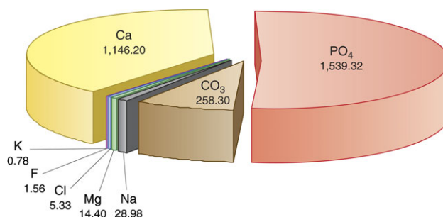
Fig. 5. Bone composition in normal individuals (in grams). Mean values from 109 human bone specimens using Trotter's estimate for total bone mass: 4459.9 g. Reproduced with permission from Pellegrino and Biltz [80].
