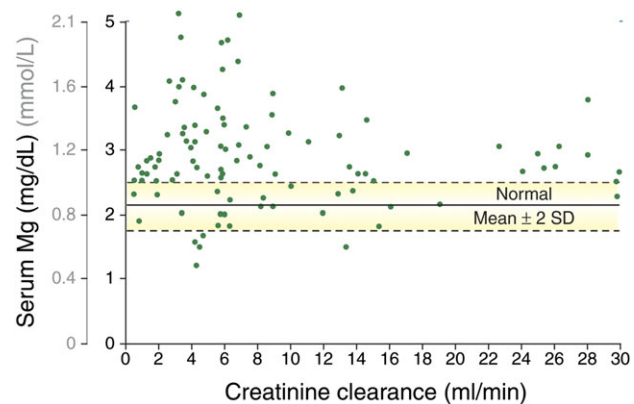
Fig. 3. The relationship between serum magnesium concentration and creatinine clearance in patients with CKD. Each point represents a result from a single patient. Normal range serum magnesium: 0.65–1.05 mmol/L (1.58–2.55 mg/dL). (With permission from Coburn et al. [12] Copyright (1969), American Medical Association. All rights reserved.)
