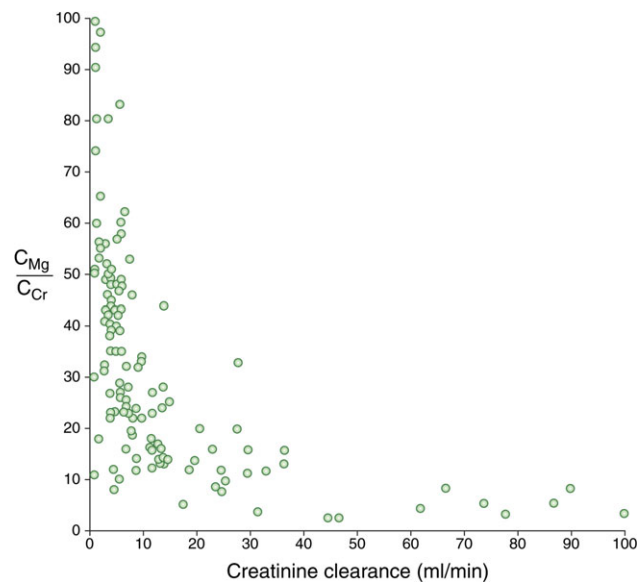
Fig. 2. The relationship between the fractional excretion of magnesium ( C_{Mg} ) and endogenous creatinine clearance ( C_{Cr} ) in patients with chronic renal disease. Each point represents a result from a single patient (With permission from Coburn et al. [12]. Copyright (1969), American Medical Association. All rights reserved.)
