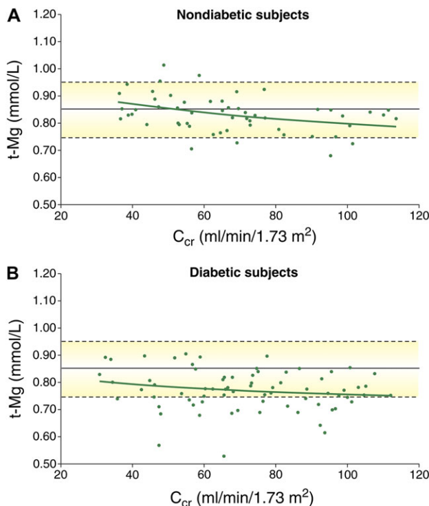
Fig. 1. Distribution of serum total magnesium (t-Mg) values as a function of creatinine clearance ( C_{Cr} ) in non-diabetic (A) and diabetic (B) patients (adapted from [11]). (Solid green line shows the course of t-Mg as predicted by regression analysis, with the reference level mean and upper/lower limits shown by solid and dotted lines, respectively.) In non-diabetic patients, serum t-Mg increased significantly when C_{Cr} decreased from 115 to 30 mL/min/1.73 m 2 , ( r = -0.38 , P < 0.001 ), whereas this was not the case in the diabetic group ( r = -0.18 , P > 0.05 ). Diabetes Care by American Diabetes Association. Copyright 2004. Reproduced with permission of American Diabetes Association in the format Journal via Copyright Clearance Center.
