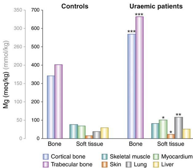
Fig. 6. Bone and tissue magnesium content in uraemic patients compared with controls [84]. Tissues were obtained from 33 patients with ESRD and 11 non-uraemic patients after death. Twenty-five of the renal patients had been dialysed for a period of ~23 months with a dialysis fluid containing 1.3 mEq/L (0.65 mmol/L) magnesium. Plasma magnesium concentrations were 2.57 \pm 0.41 mEq/L ( 1.29 \pm 0.21 mmol/L). Most of the controls had died in road traffic accidents. Their plasma magnesium concentrations were 1.57 \pm 0.08 mEq/L ( 0.79 \pm 0.04 mmol/L). The soft tissue samples were dried and defatted. The result is given as milliequivalent per kilogram fat-free dry solids. For myocardium, skin and lung, mean magnesium concentrations were significantly higher in uraemic patients; there was no difference for skeletal muscle or liver. The bone was defatted and then dried. Results are given as milliequivalent per kilogram ashed weight. Although the mineral content of uraemic trabecular bone was decreased by 8% and of cortical bone by 5%, there was still a significant increase in bone magnesium content on a dry weight basis in uraemic patients (* P < 0.01 ; ** P < 0.0005 ; *** P < 0.0001 versus controls) (2 mEq/L = 1 mmol/L). Reproduced with permission from Contiguglia et al. [84].
